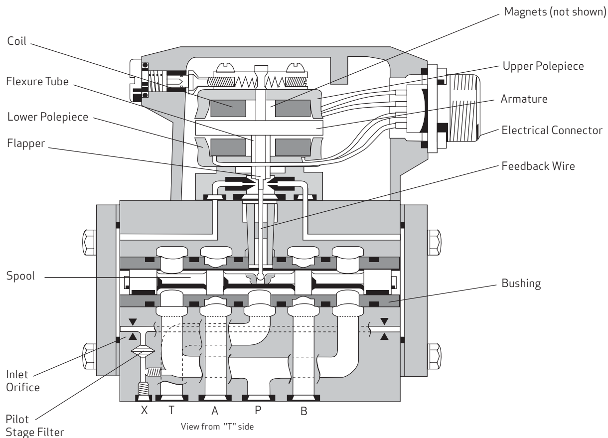
Electro-hydraulic Servo Valve Cut-away
