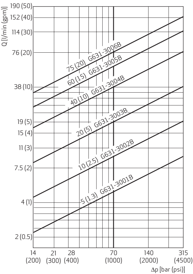
Flow Diagram
