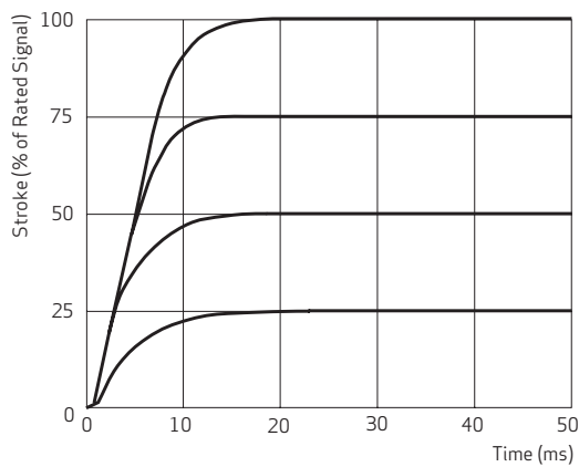
Step Response
